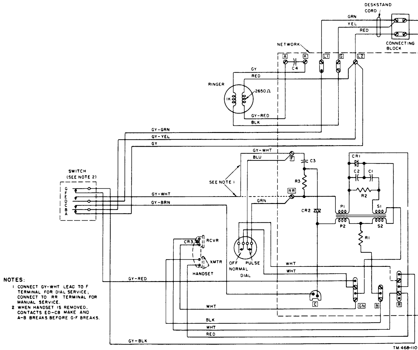
Figure 67. Telephone TA-236/PT, dial, wiring.
