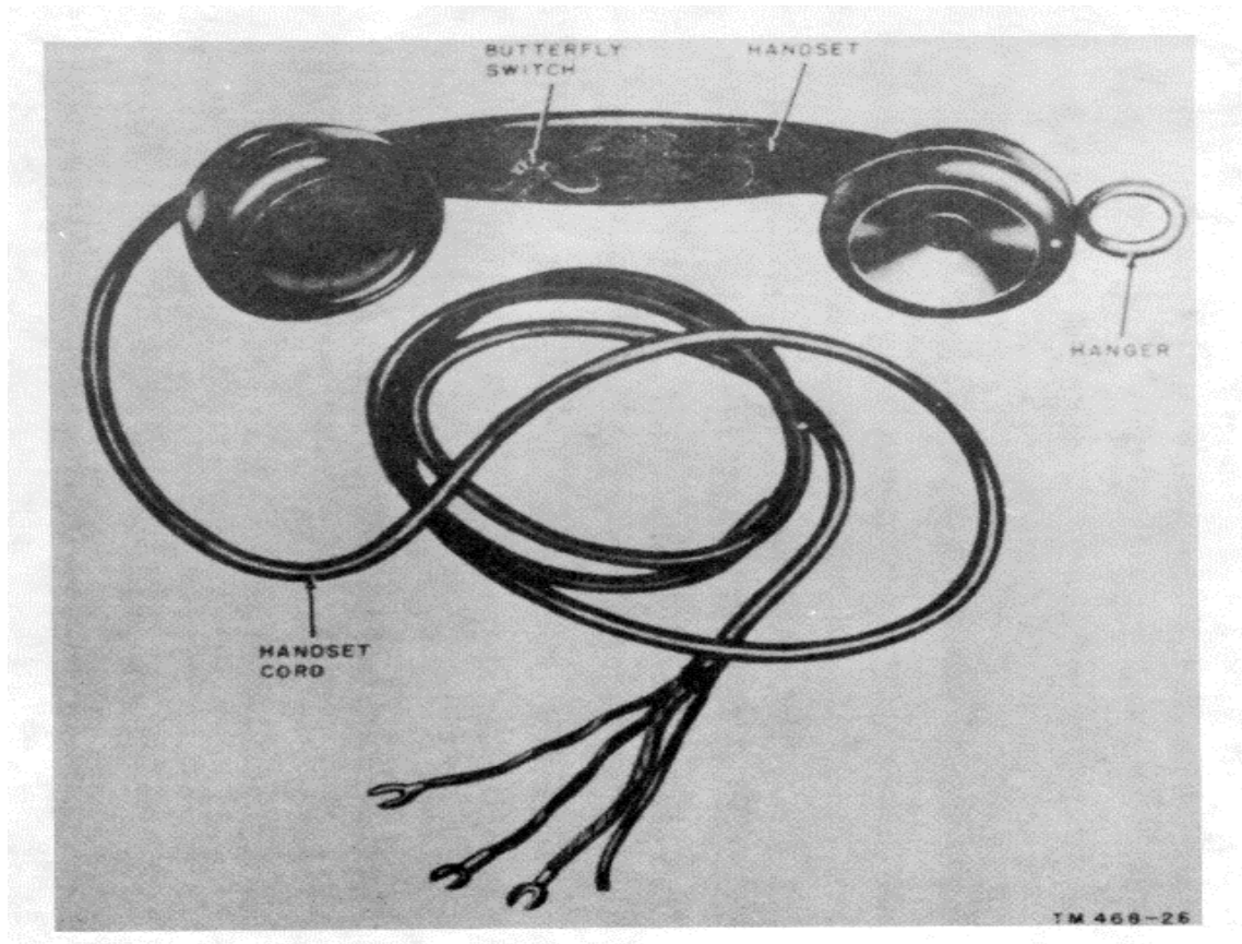
Figure 26. Handset TS-12-F.
