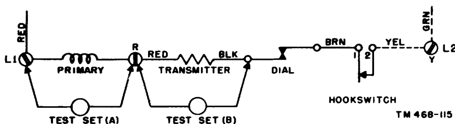
Figure 76. Telephone TP-A, test for short-circuited primary winding and transmitter, wiring diagram.
