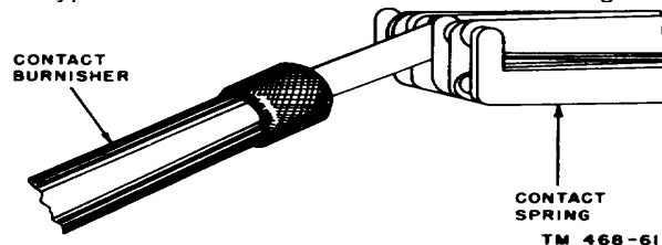
Figure 88. Cleansing contacts with contact burnisher.
