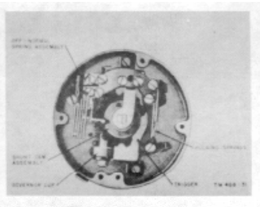
Figure 31. Dial TA-45/IGT (Telephonic), rear view, showing location of parts.
