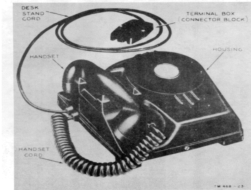
Figure 22. Telephone TA-166/U, arranged for manual operation.
