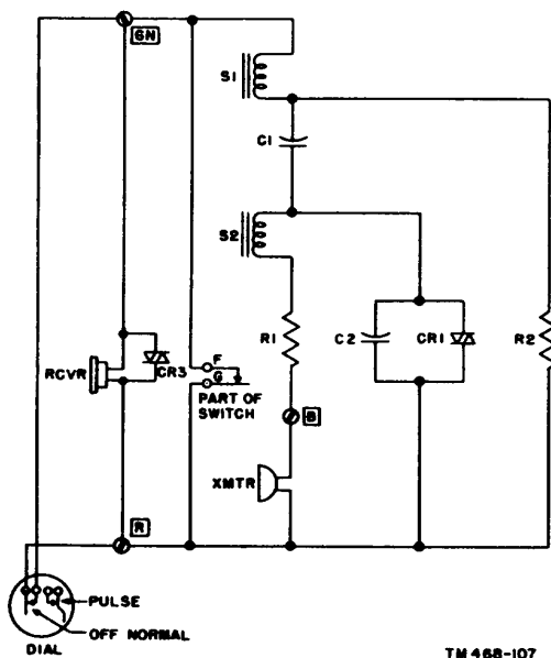
Figure 64. Receiver circuit, dial, schematic.
